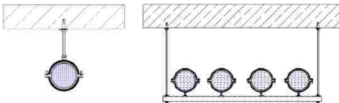
Plumbing pipe support from PEB Structure
